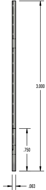
RIGHT VIEW
