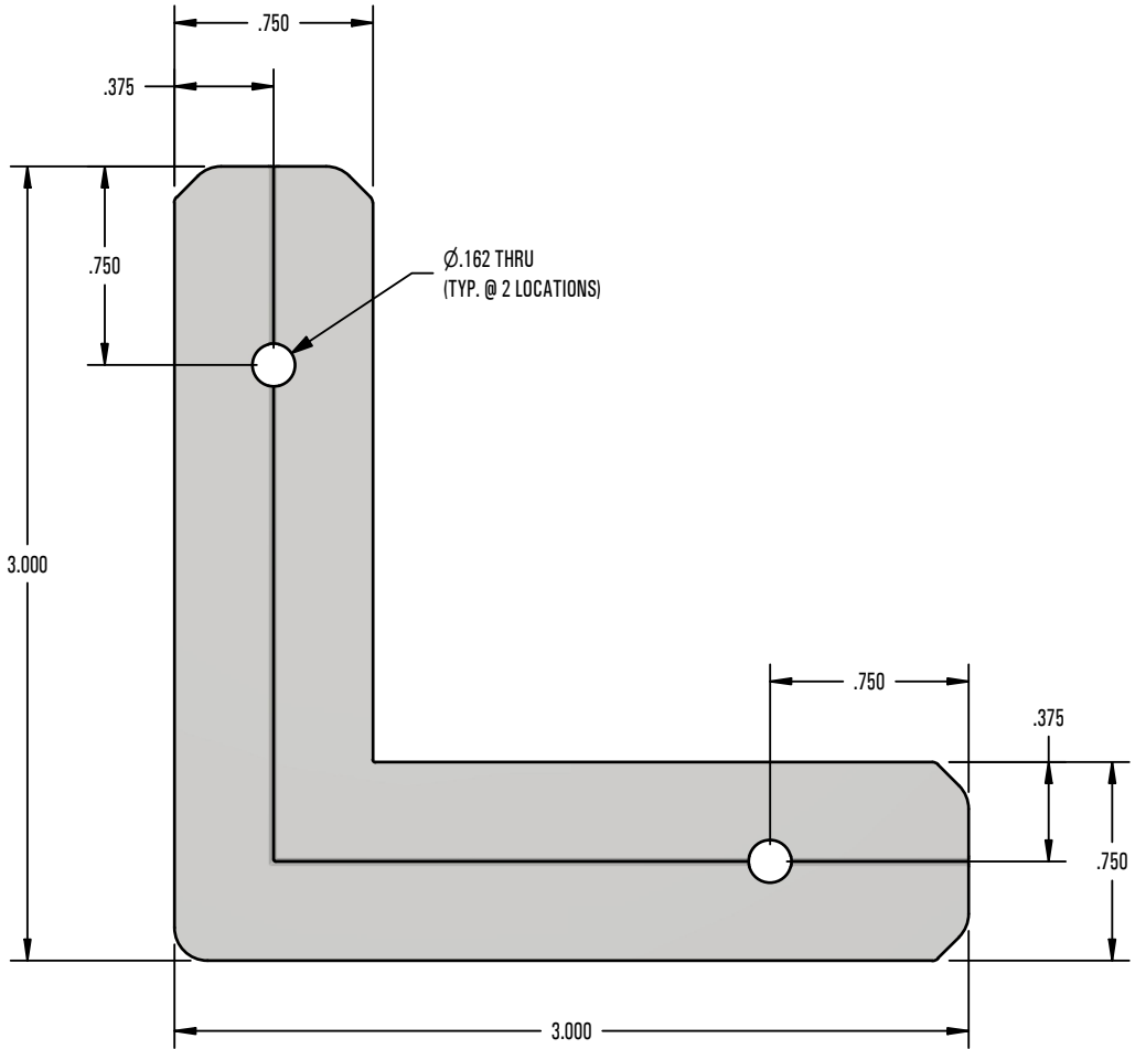
FRONT VIEW
