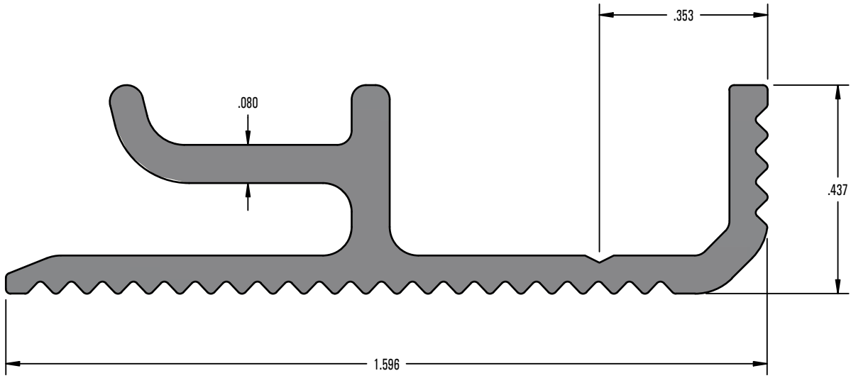
PROFILE VIEW
