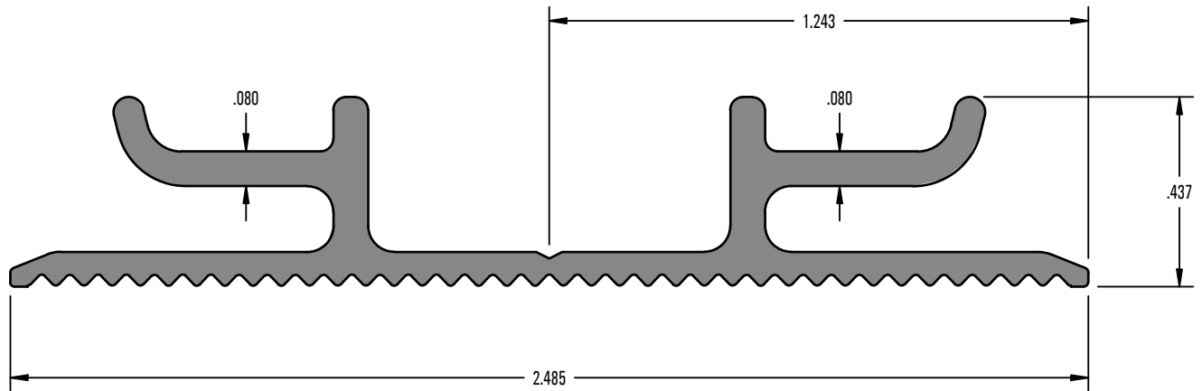
PROFILE VIEW
