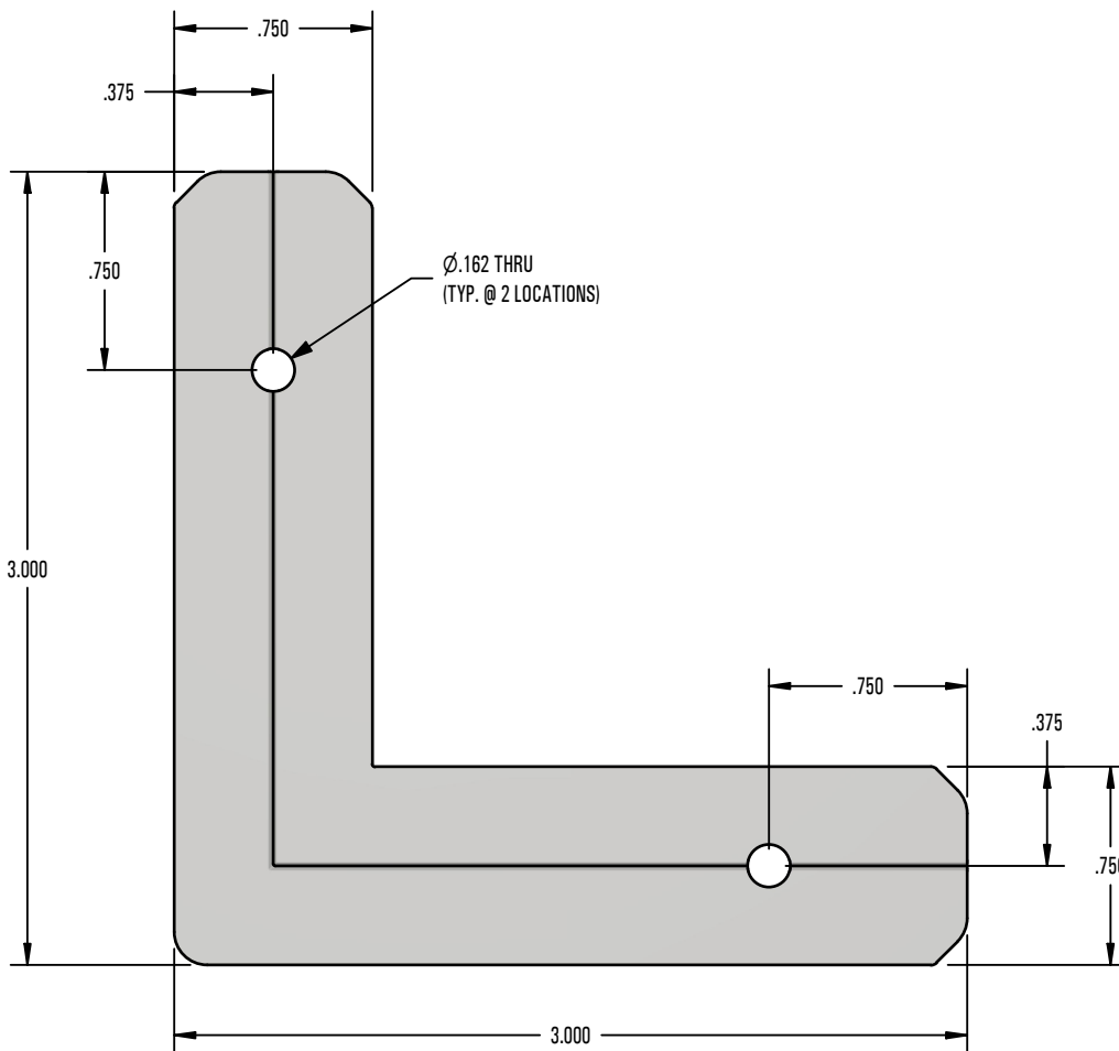
FRONT VIEW
