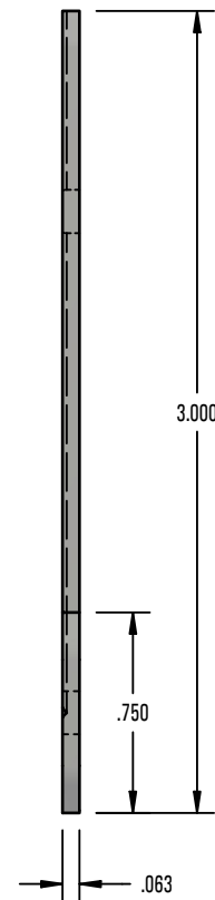
RIGHT VIEW
