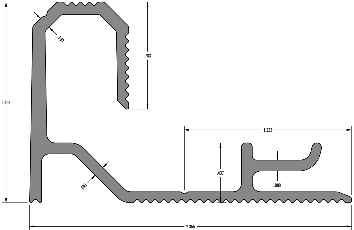
PROFILE VIEW
