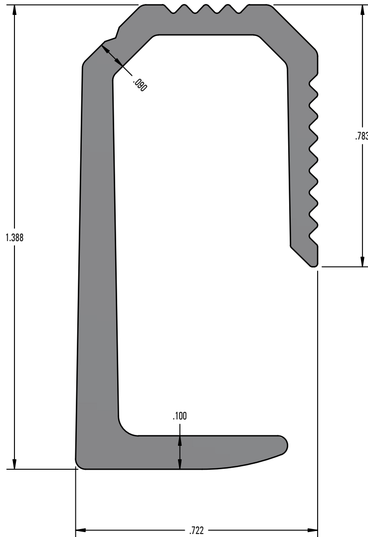
PROFILE VIEW
