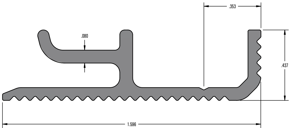
PROFILE VIEW
